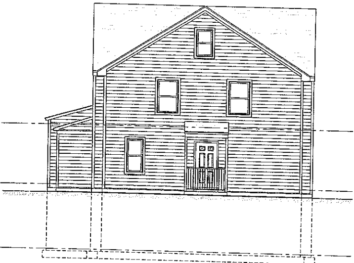
3 REAR ELEVATION SCALE: 1/4" = 1'-0"
