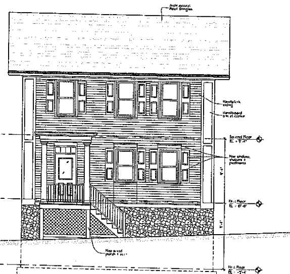
① FRONT ELEVATION SCALE: 1/4" = 1'-0"
