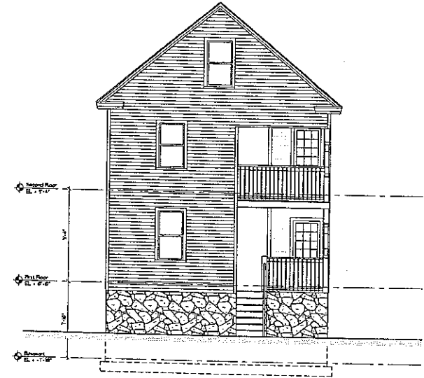
③ REAR ELEVATION SCALE: 1/4" = 1'-0"
