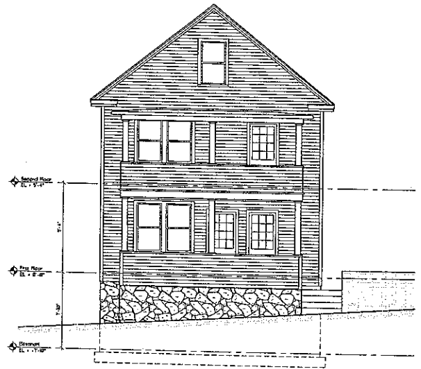
① FRONT ELEVATION SCALE: 1/4" = 1'-0"
