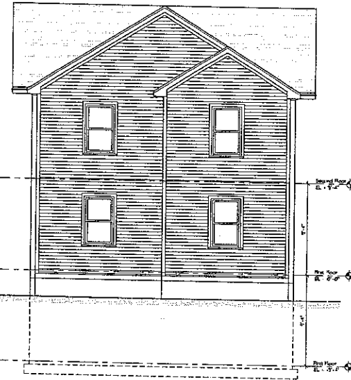
③ REAR ELEVATION SCALE: 1/4" = 1'-0"
